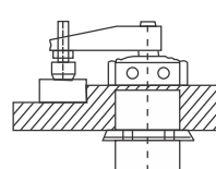
with grooved nut from below
